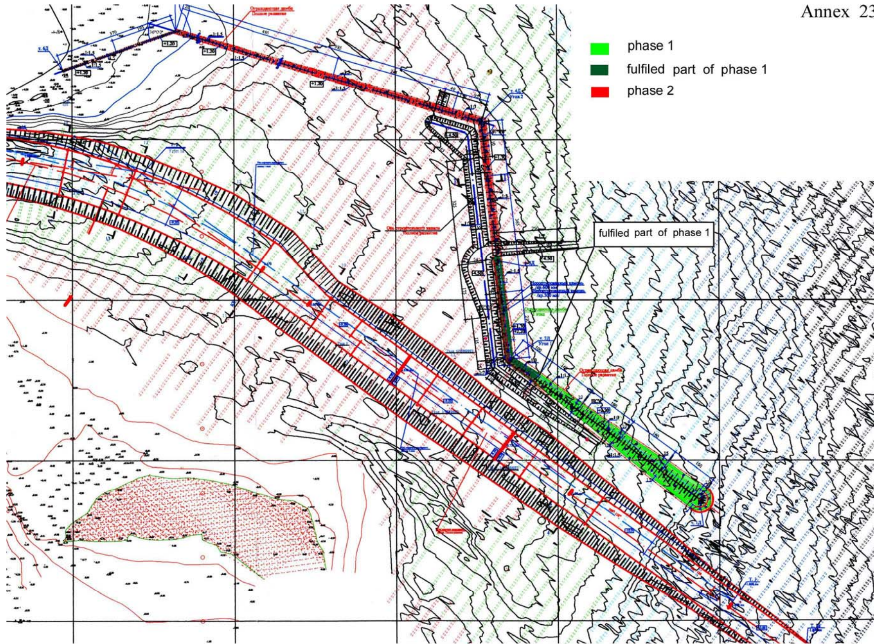
Scheme of Retaining dam for seaward access channel
